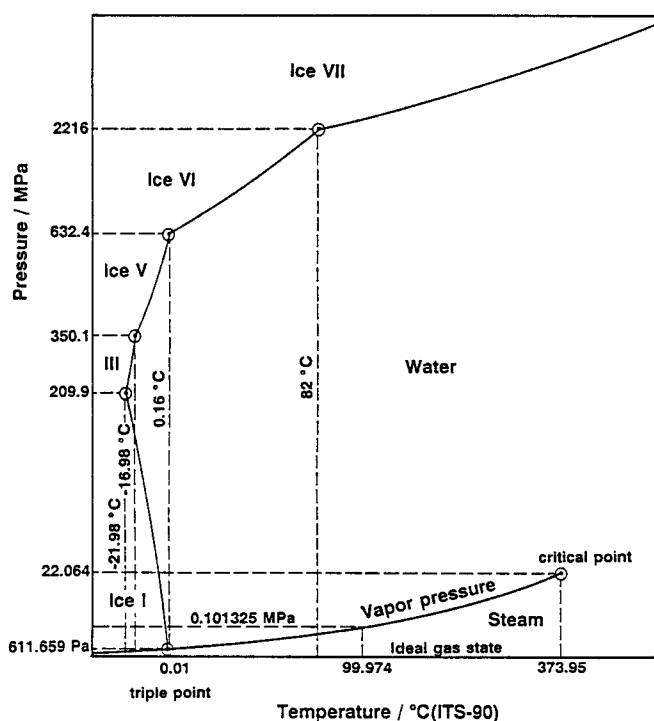
FIG. 1. Phase boundaries for ice, water, and steam.
