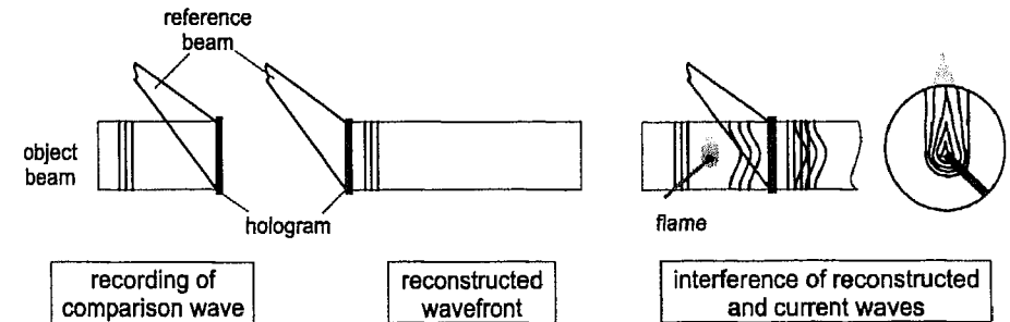
Figure 9. Real-time method for holographic interferometry
