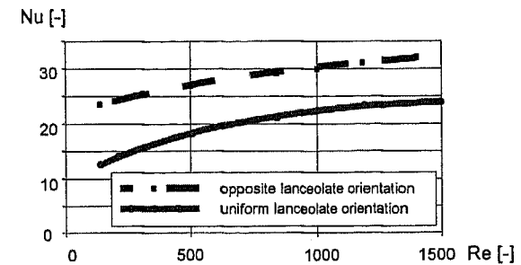
Figure 13. Average Nusselt numbers in cross-flow bundles with lanceolate tubes
