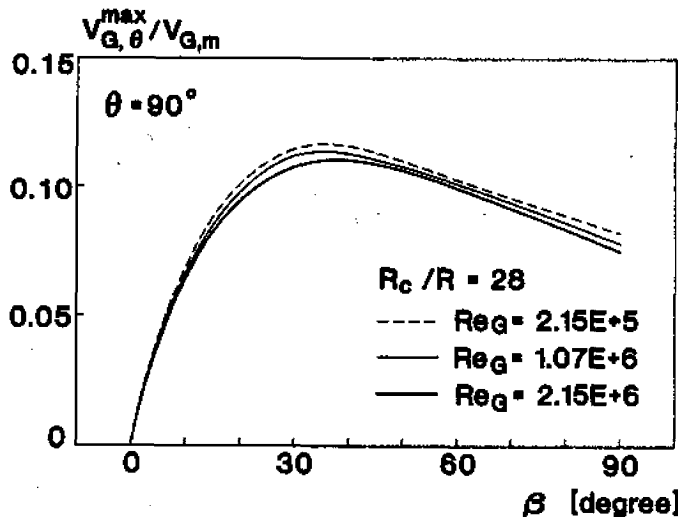
Figure 7. Influence of Reynolds number on the secondary flow.
