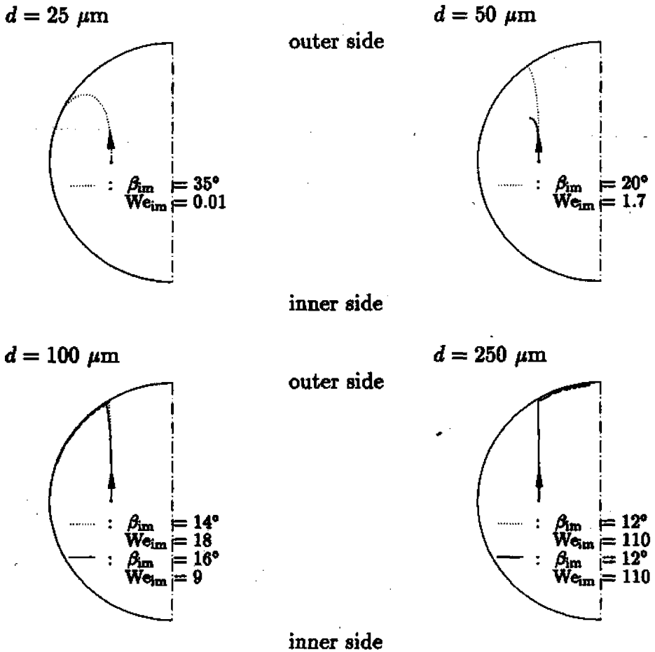
Figure 9. Droplet motion under thermal effect: R_c/R = 42 , Re_0 = 1.07 \times 10^6 , q_w = 60 \text{ kW/m}^2 , T_{Q,0} - T_s = 80^\circ\text{C} .
