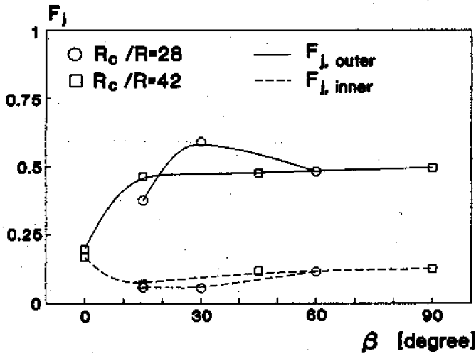
Figure 14. Effect of curvature ratio on the phase distribution: G = 680 \text{ kg/m}^2 , q_w = 20 \text{ kW/m}^2 .
