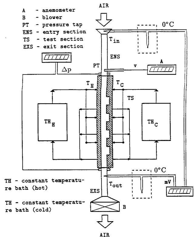
Figure 2. The experimental setup
