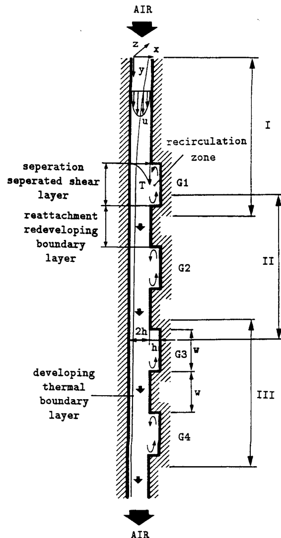
Figure 1. Schematic of the grooved geometry and the flow situation
