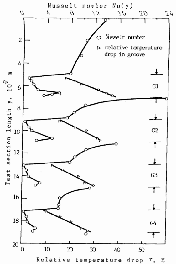
Figure 5. Local Nusselt number and relative temperature drop inside the groove compared to total temperature drop vs. y for \Delta T = 45 K and Re = 1220.8
