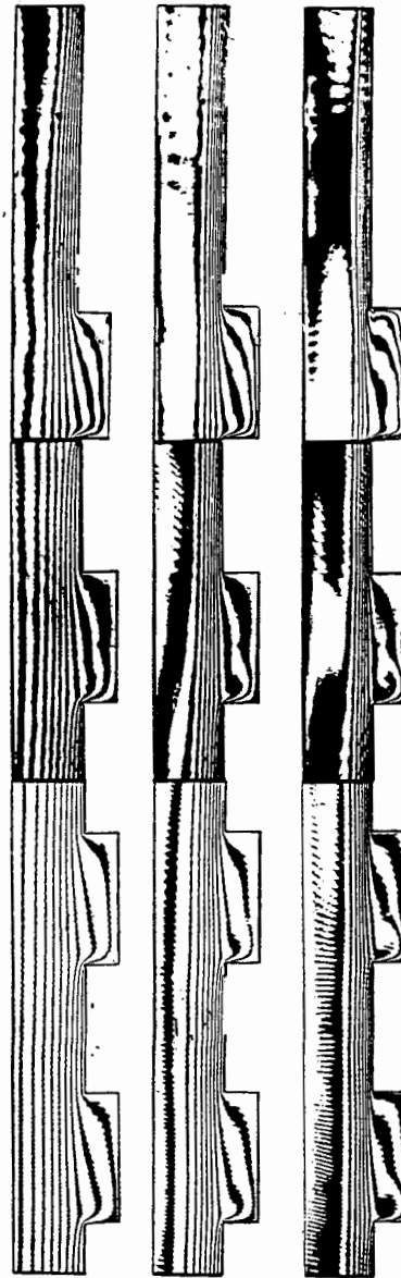
Figure 3. Interferogram sets for \overline{\Delta T}=30 K and Re=293 , Re=604 and Re=1561 , taken by infinite fringe field technique
