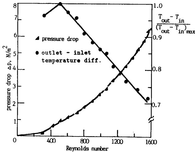
Figure 6. Pressure drop and temperature increase in test section vs. Reynolds number
