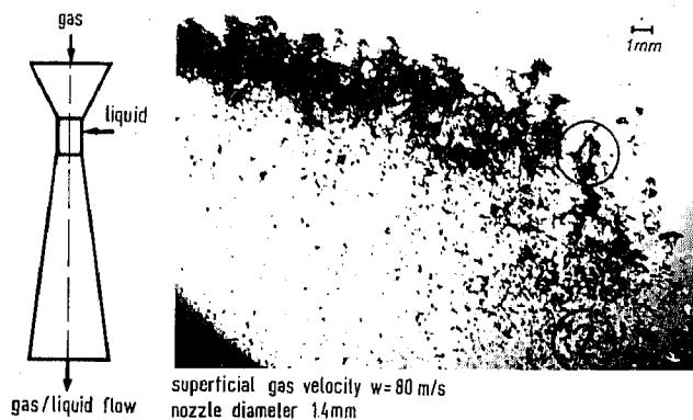
Fig. 3. Jet break-up (Photographic survey).
