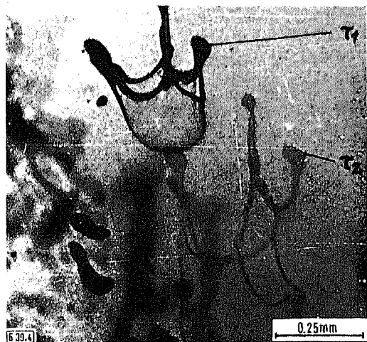
Fig. 4. Parachute like sheet (zone "1"). \tau_2 - \tau_1 = 10^{-5} s
