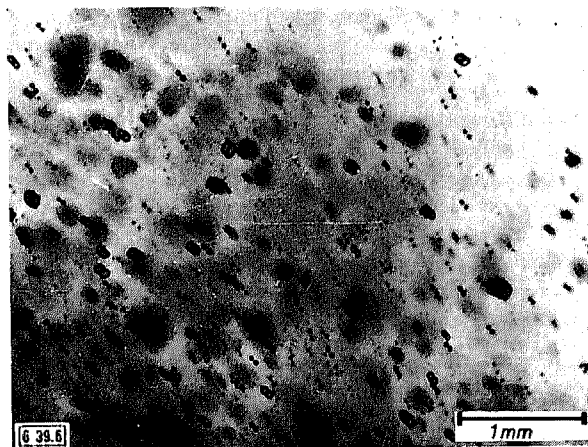
Fig. 6. Droplets at the end of the atomization zone.
