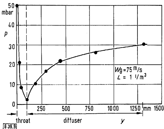
Fig. 9. Pressure distribution in a Venturi-scrubber.
