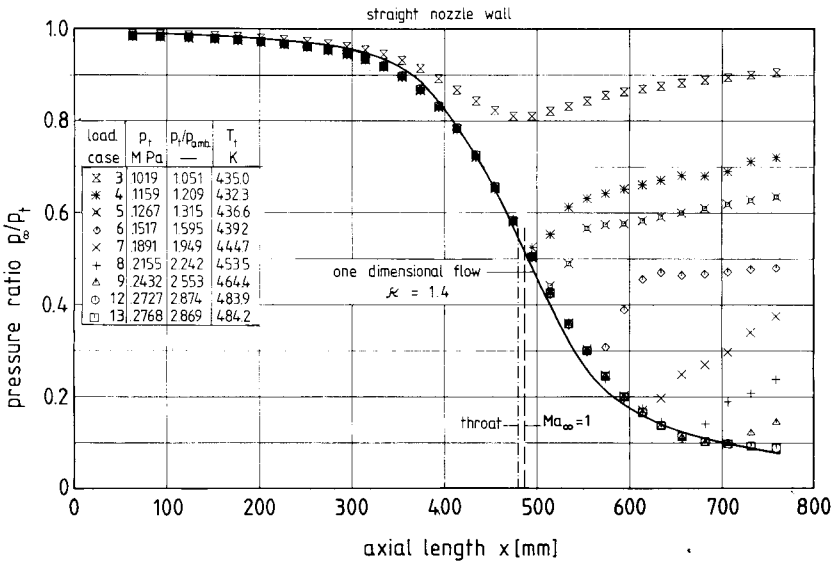
FIG. 5. Static-to-total pressure ratio p_{0\infty}/p_t vs axial length x .
