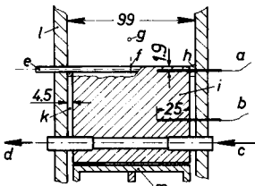
a = thermocouple b = thermocouple c = cooling water entry d = cooling water exit e = static pressure tapp. f = static pressure hole g = flow cross section h = rubber sealing i = segment (copper) k = air gap l = slab m = frame
