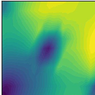
Reference \psi
