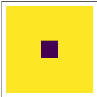
Reference \psi
