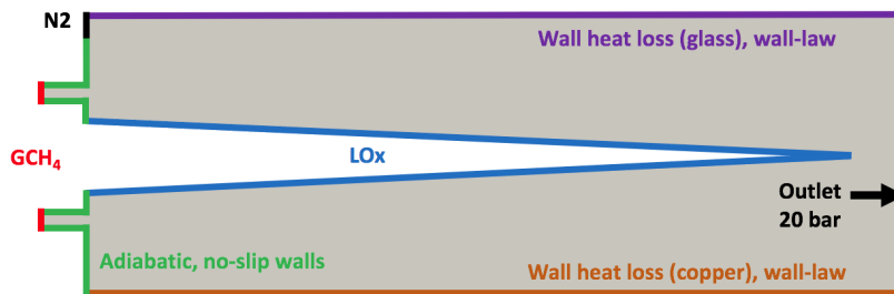
FIGURE 8. Boundary conditions
