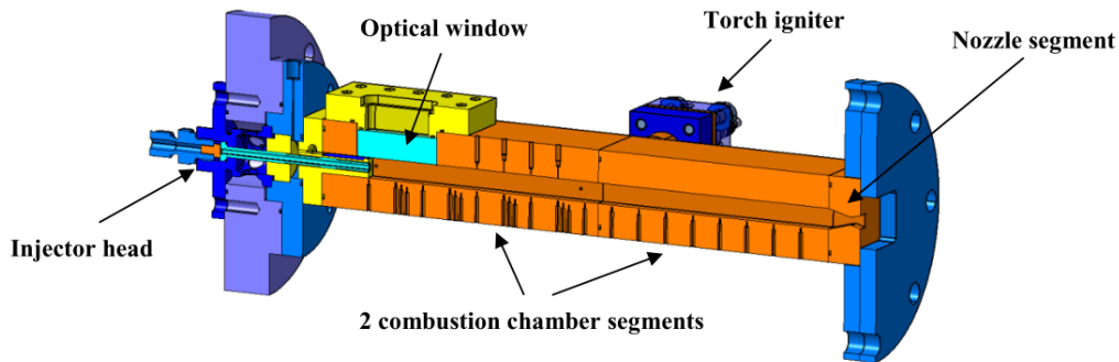
FIGURE 5. Combustion chamber with cryogenic injector head and optical access window [12]
