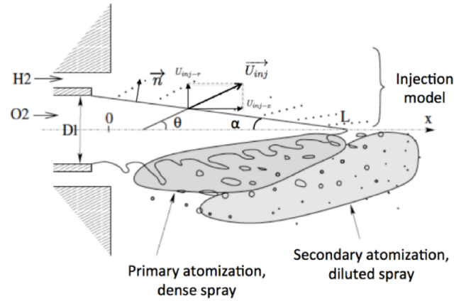
FIGURE 7. LOx atomization model overview (from [27])
