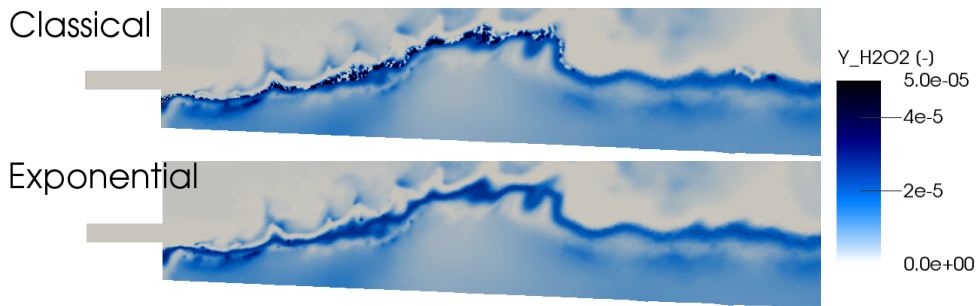
FIGURE 10. \text{H}_2\text{O}_2 mass fraction instantaneous field near the liquid cone. Top: classical integration. Bottom: exponential integration.
